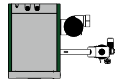
Variant D: Flue pipe connection on the right Pellet insertion on the right
