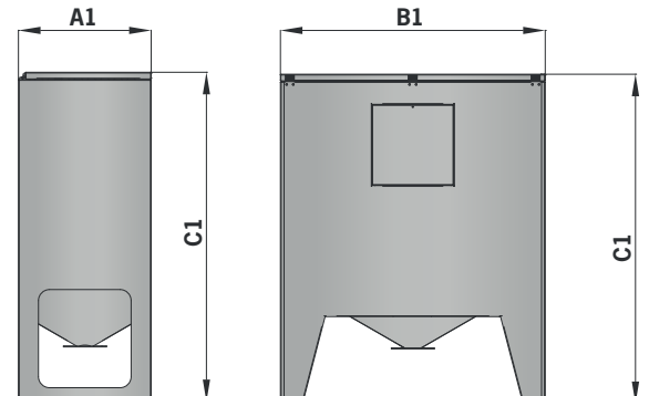
Hand filling hopper FLEX 740
