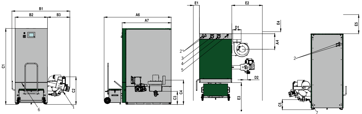
Illustration: pellet insertion on the right side - optionally also available on the left side
