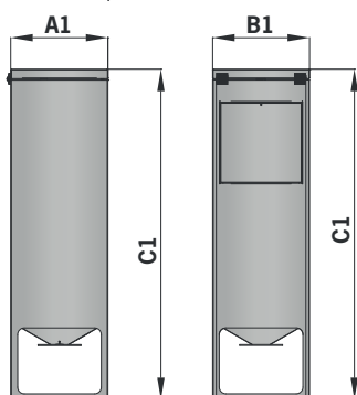
Hand filling hopper FLEX 225
